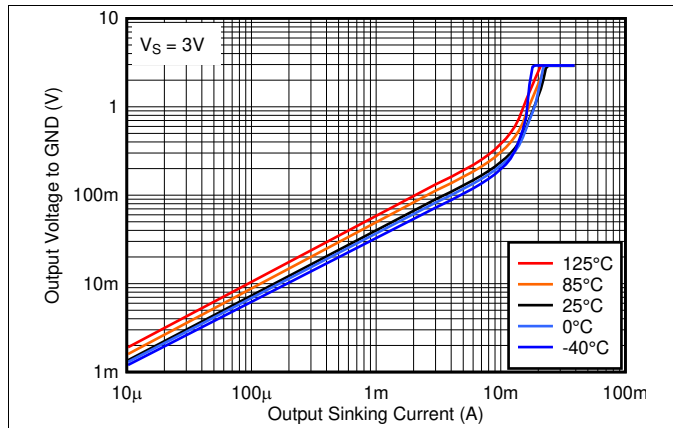
Figure 24. Output Low Voltage vs. Output Sinking Current at 3V
