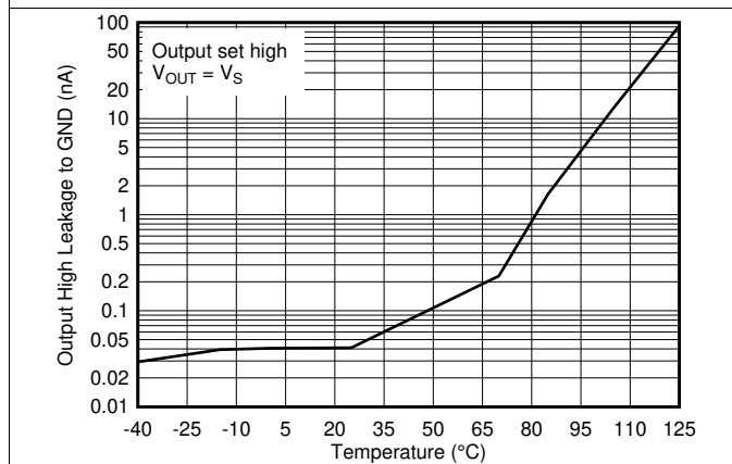
Figure 28. Output High Leakage Current vs. Temperature at 5V
