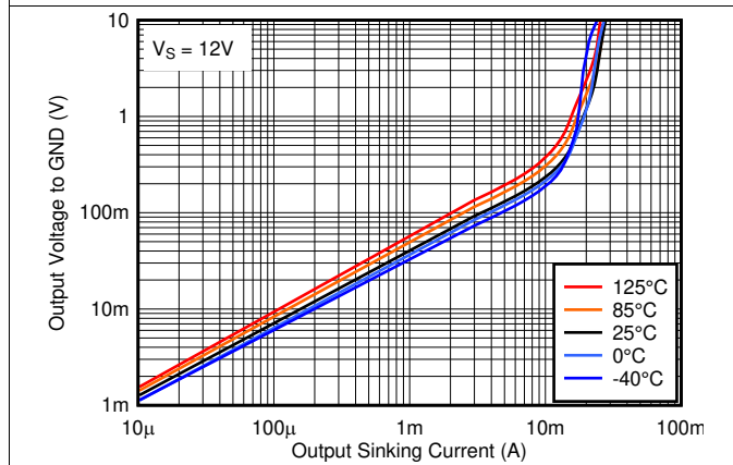
Figure 26. Output Low Voltage vs. Output Sinking Current at 12V
