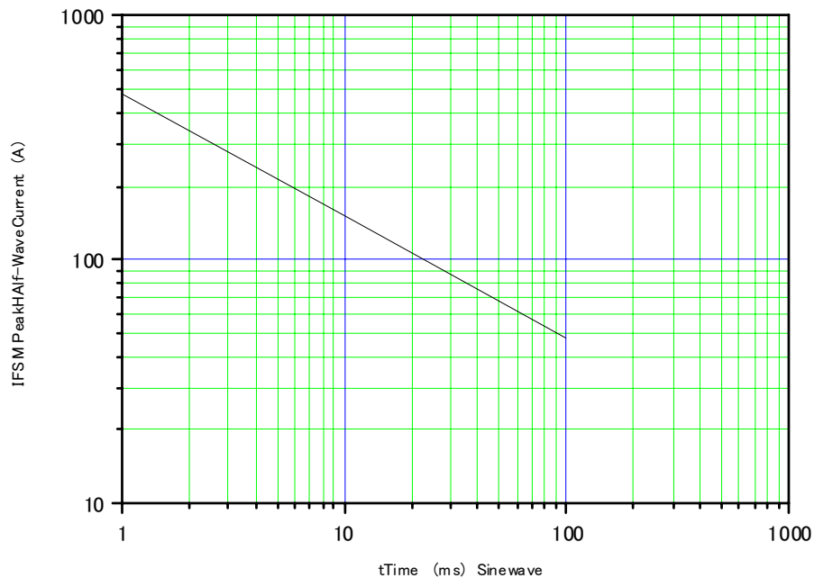
Surge Current Ratings (max.)
