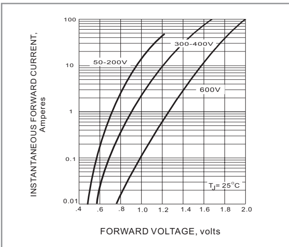
Fig. 3 FORWARD CHARACTERISTICS
