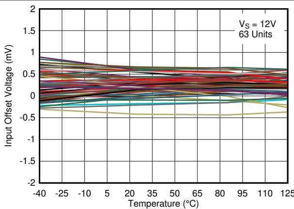
图 6-20. Input Offset Voltage vs. Temperature at 12V
