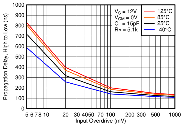
图 6-30. High to Low Propagation Delay vs. Input Overdrive Voltage, 12V
