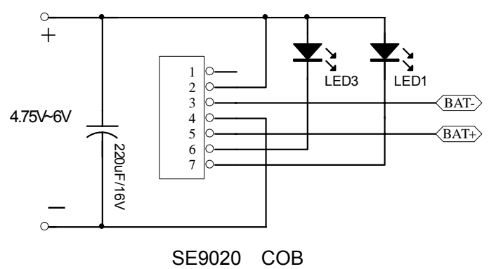
Figure 6 2 LED circuit
