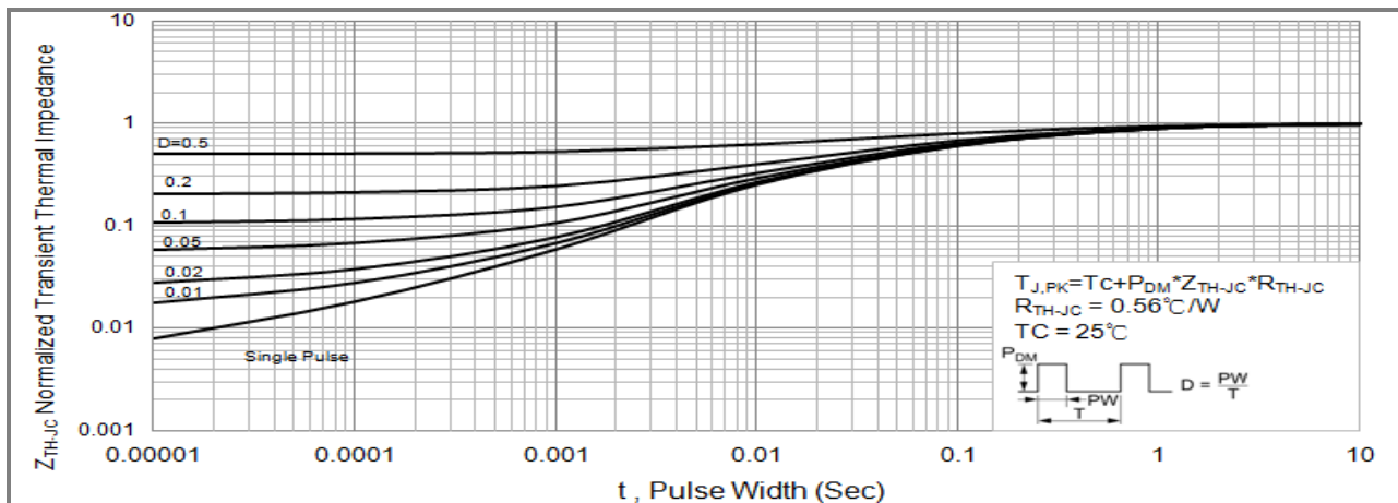
Fig.13 PJP12NA60 Normalized Transient Thermal Impedance vs. Pulse Width
