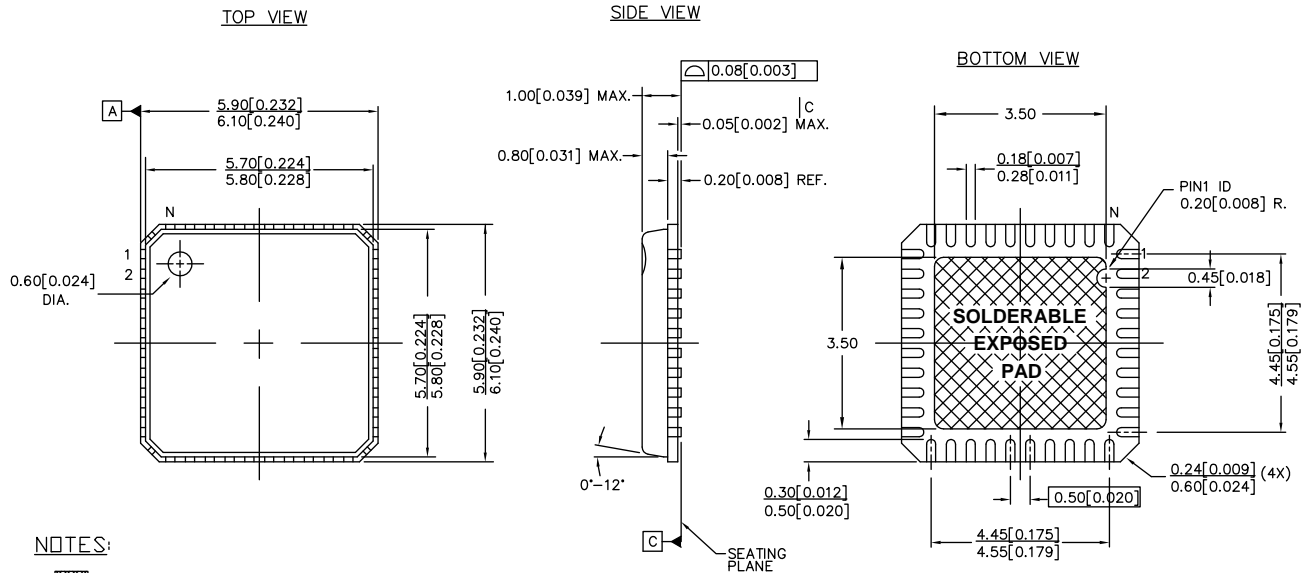
Figure 12. 40-Pin Pb-free QFN 6 × 6 mm
